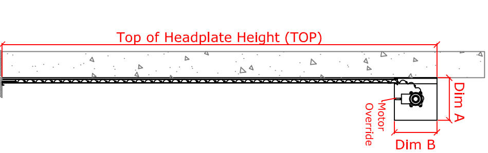
Section View Rolling Back to Front (B/F)
